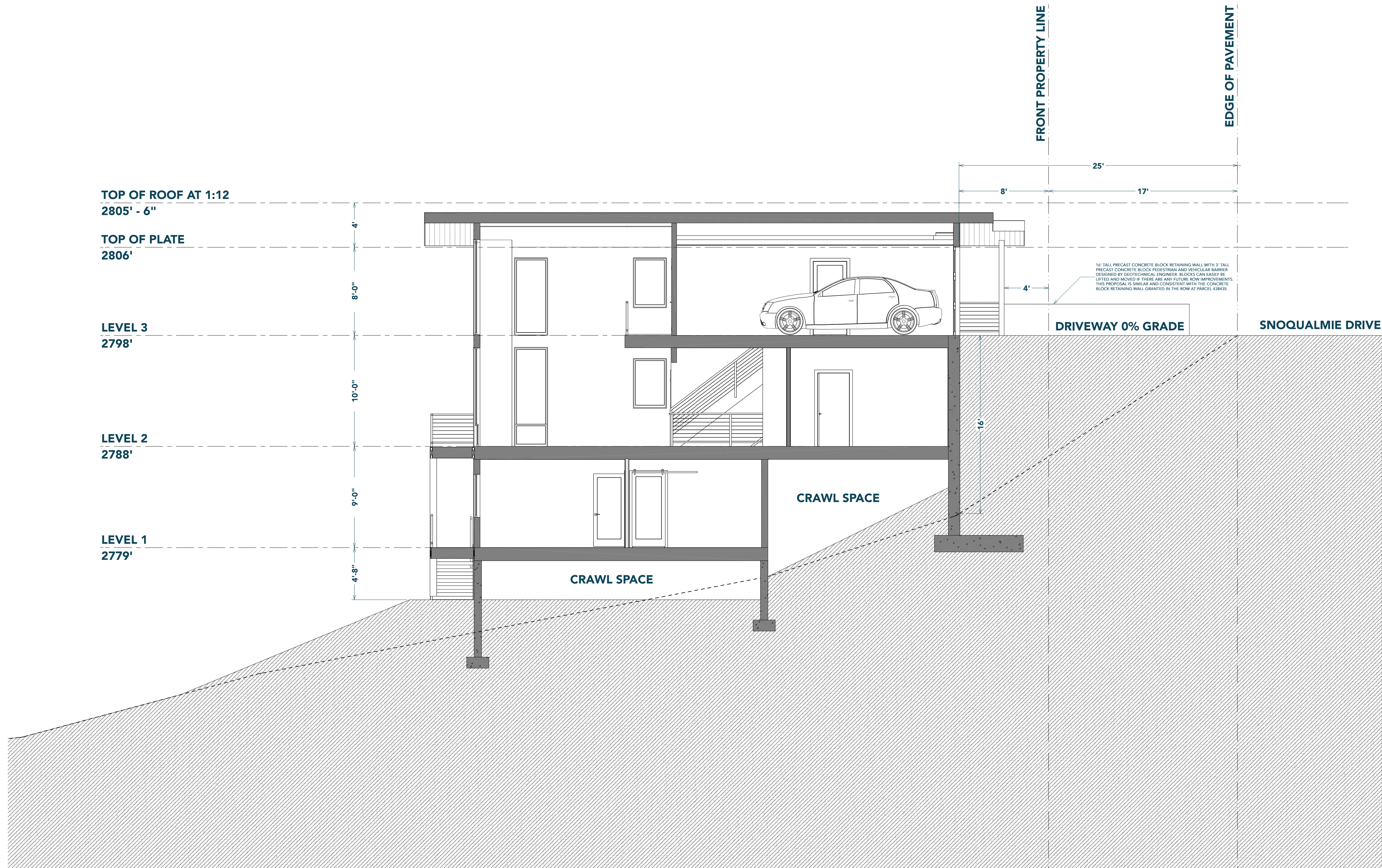
DIAGRAMATIC SECTION OF SCHEMATIC DESIGN
